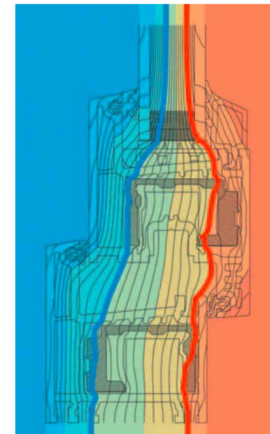
Thermograph of a window with Kömmerling profiles.
